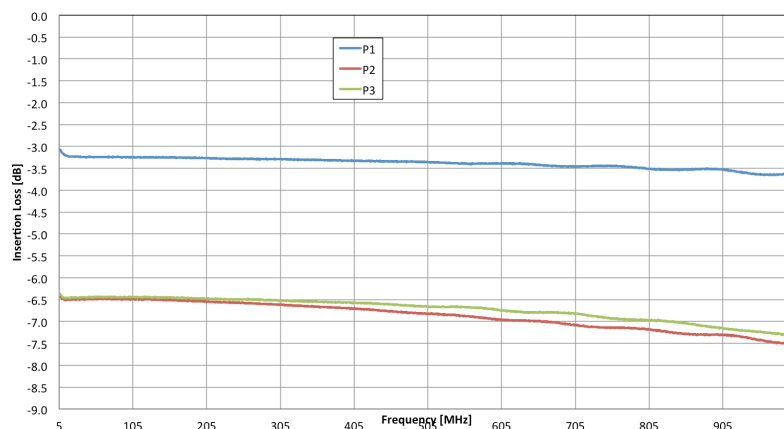
PPC-GHS-3E, Insertion Loss
