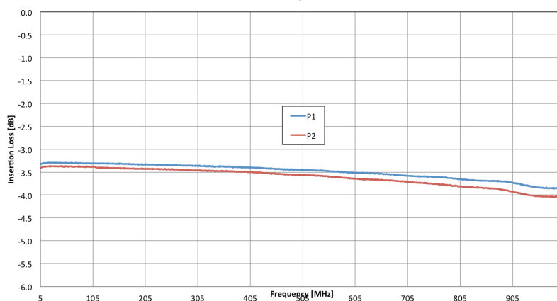
PPC-GHS-2E, Insertion Loss
