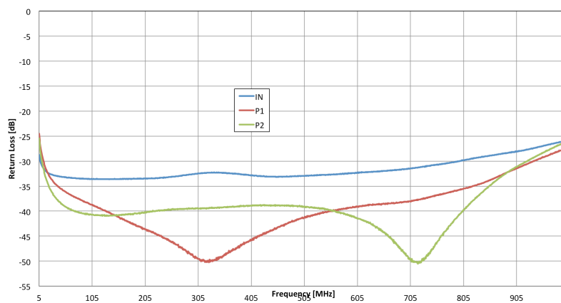
PPC-GHS-3E, Return Loss
