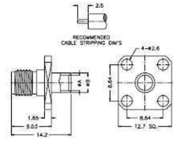
Solder 4-Hole Flange Straight Jack Termination Instruction B
