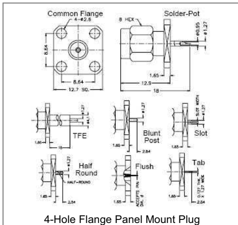
4-Hole Flange Panel Mount Plug
