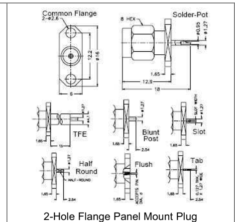
2-Hole Flange Panel Mount Plug
