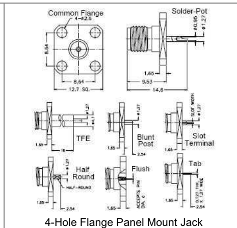
4-Hole Flange Panel Mount Jack
