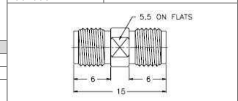
Jack to Jack Adapter
