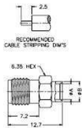
Solder Straight Jack Termination Instruction B
