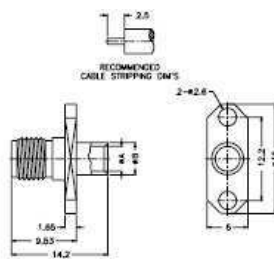
Solder 2-Hole Flange Straight Jack Termination Instruction B
