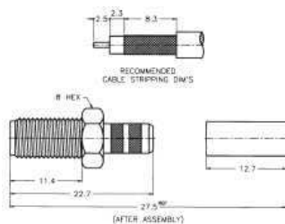
Crimp/Crimp Non-Captive Contact Str. Jack Termination Instruction E
