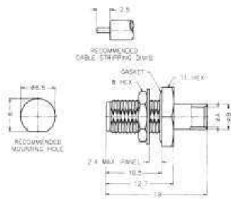
Solder Bulkhead Straight Jack Termination Instruction B
