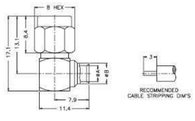
Solder Right Angle Plug Termination Instruction D
