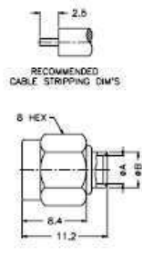
Solder Straight Plug with Contact Termination Instruction B
