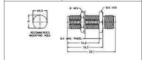
Jack to Jack Bulkhead Adapter
