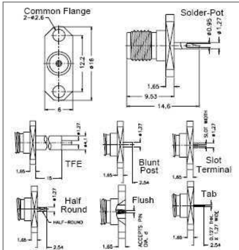
2-Hole Flange Panel Mount Jack
