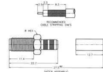
Crimp/Crimp Non-Captive Contact Str. Jack Termination Instruction E
