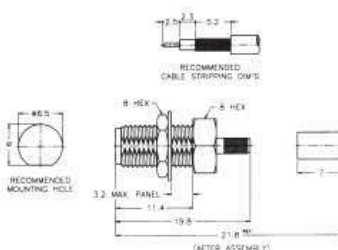
Crimp/Crimp Bulkhead Non-Captive Contact Str. Jack Termination Instruction E
