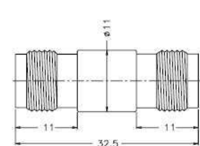
Jack-to-Jack Straight Adapter
