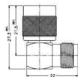
Plug-to-Jack Right Angle Adapter
