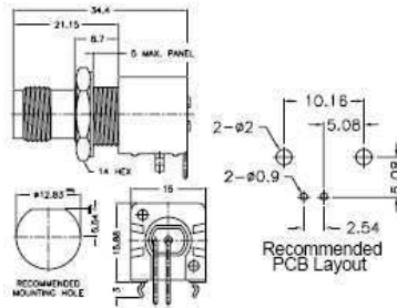
PCB Mount Right Angle Plastic Jack
