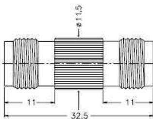
Jack-to-Jack Straight Adapter
