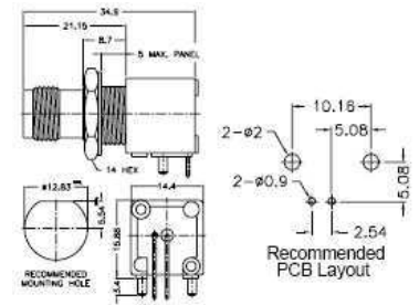
PCB Mount Right Angle Metal Jack
