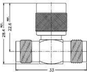
Jack-to-Plug TEE Adapter
