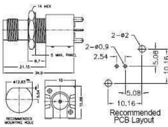
PCB Mount Straight Plastic Jack
