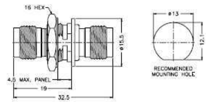
Jack-to-Jack Straight Bulkhead Adapter Isolated from Ground
