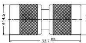
Plug-to-Plug Straight Adapter
