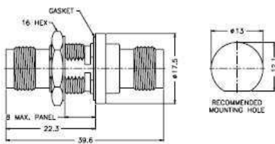
Jack-to-Jack Straight Bulkhead Adapter
