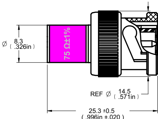
DIM OUTLINE
