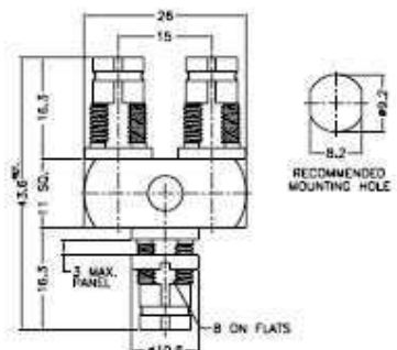
Jack to Jack to Jack 'Y' Link Adapter
