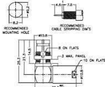
Clamp/Solder Right Angle Bulkhead Jack Termination Instruction Q
