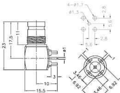
Right Angle Bulkhead Jack for PCB
