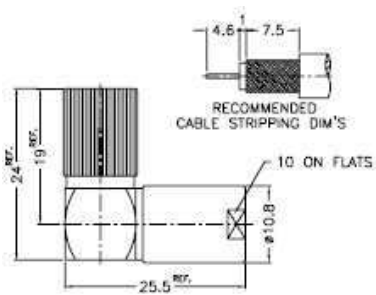
Clamp/Solder Right Angle Plug Termination Instruction Q
