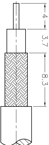
RECOMMENDED CABLE STRIPPING DIM'S
